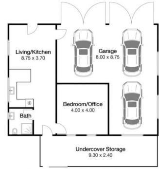
Bottom Floor (Studio/Garage)
