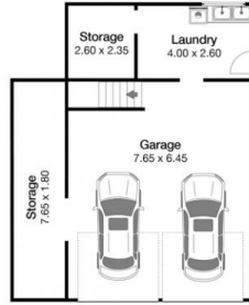
Bottom Floor
